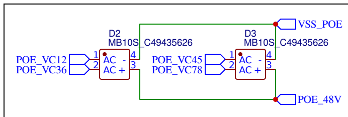
PoE AC-DC conversion
