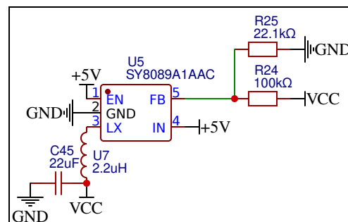
Buck Converter - 3.3V
