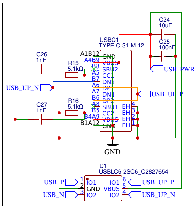
Type-C Port
