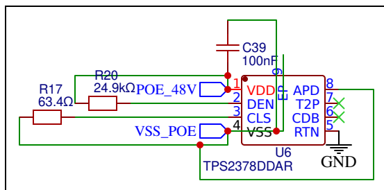
PoE Negotiation Chip
