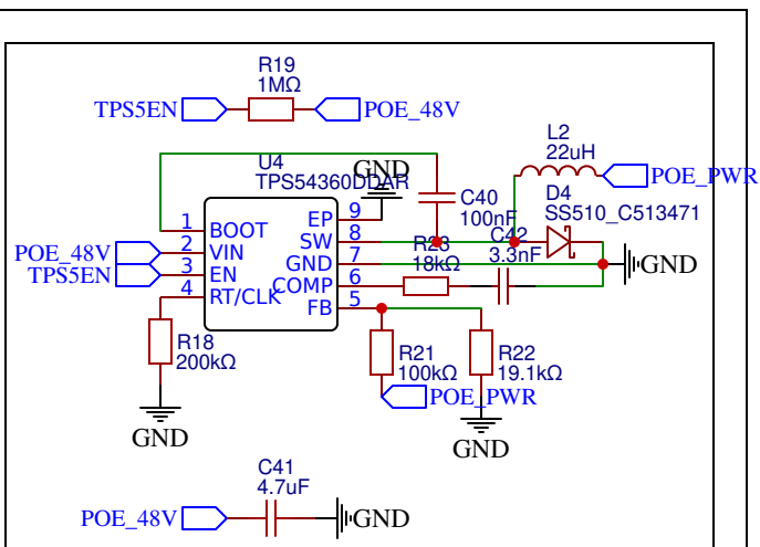
Buck Converter Chip
